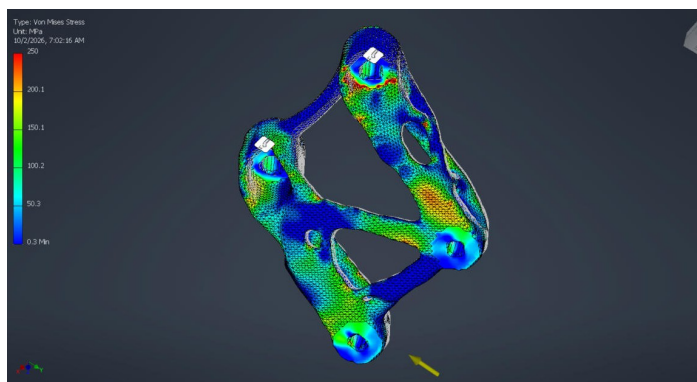
Autodesk Inventor Stress Analysis, von Mises, 5 kN remote load. Sculpted v4 shape.
