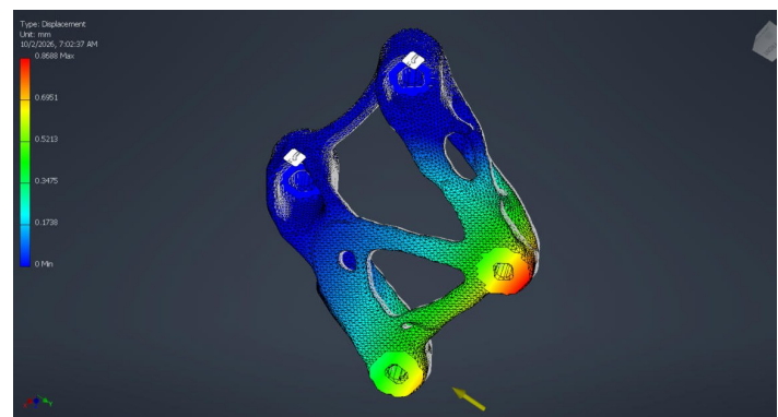
Displacement at 5 kN. Max 0.87 mm at the peg mount.
